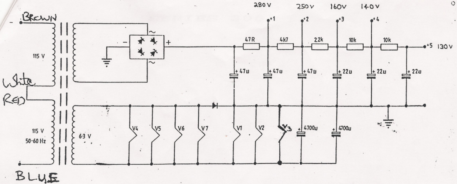
SERIES 300 POWER SUPPLY
